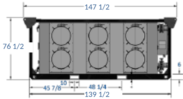
Six 20" Return Air Connections
